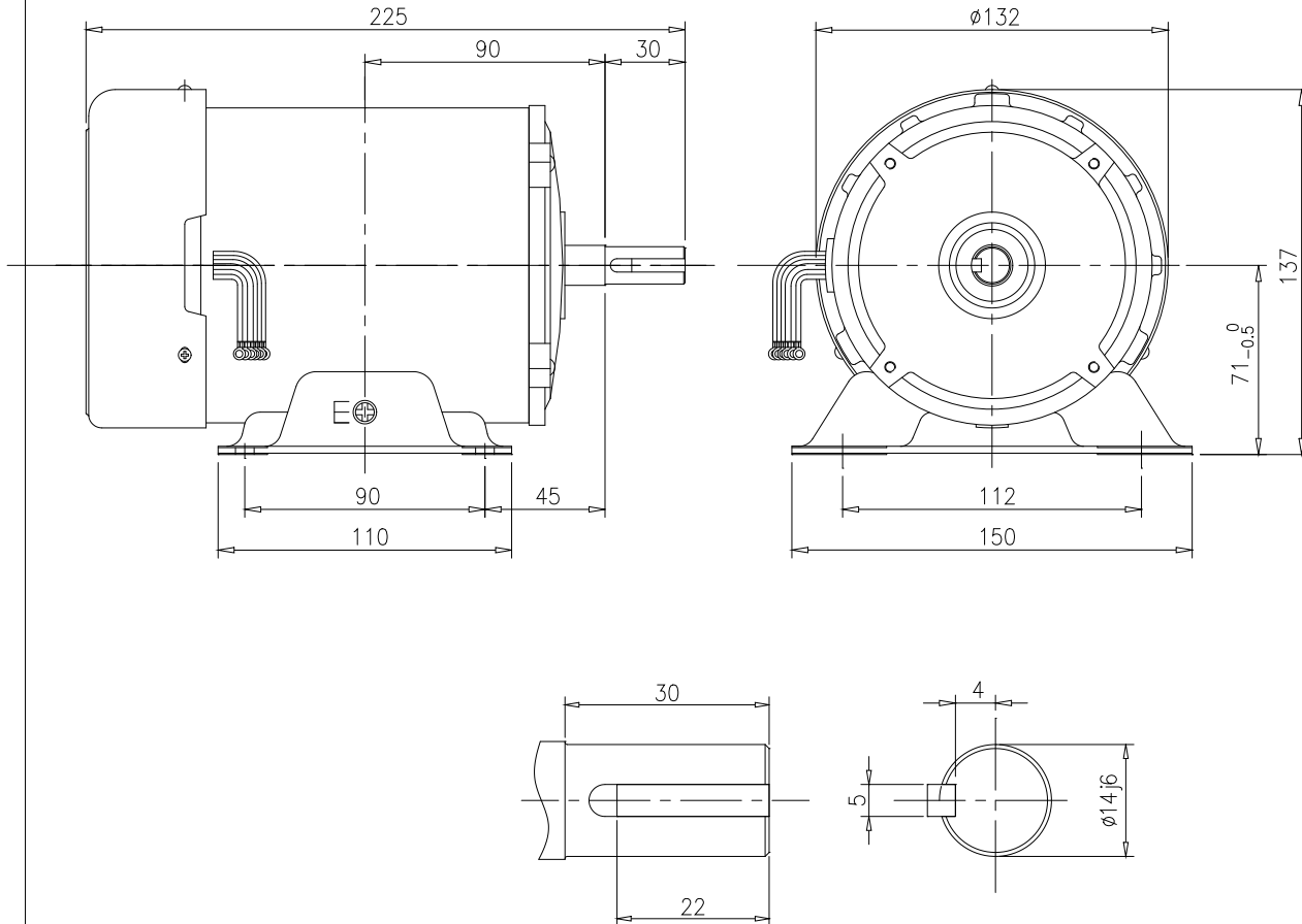
SHAFT EXTENSION
