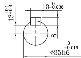
SHAFT EXTENSION
