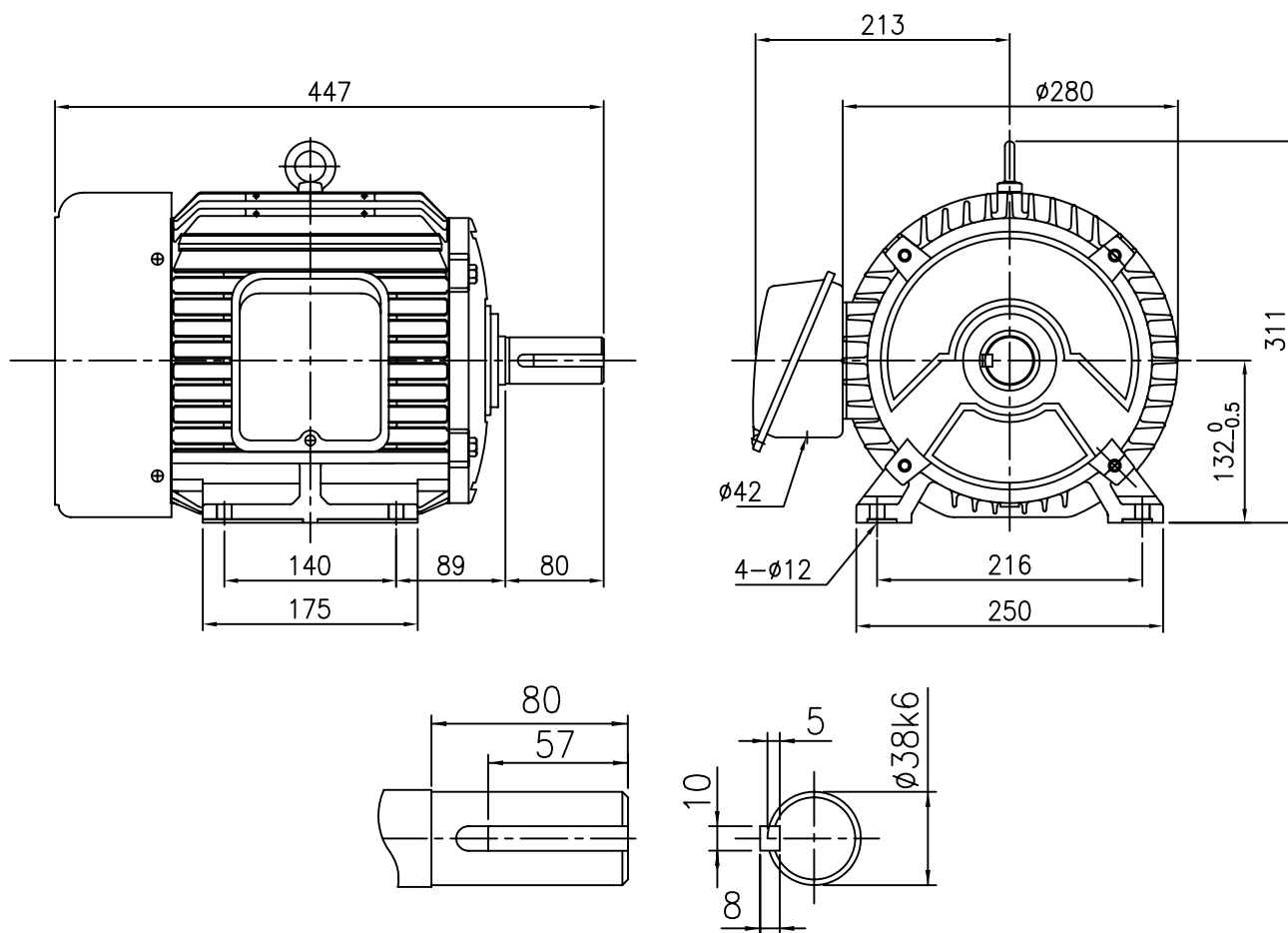
SHAFT EXTENSION
