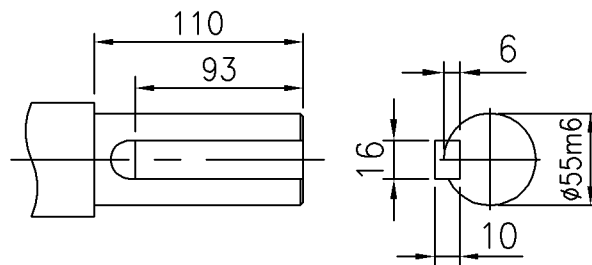
SHAFT EXTENSION
