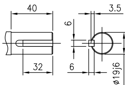
SHAFT EXTENSION
