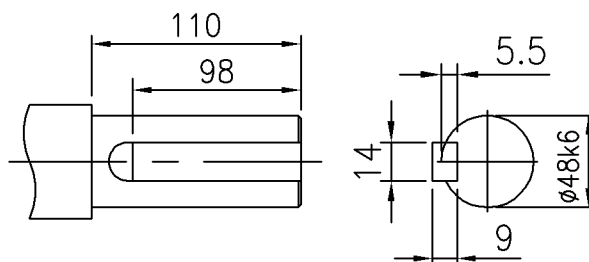
SHAFT EXTENSION
