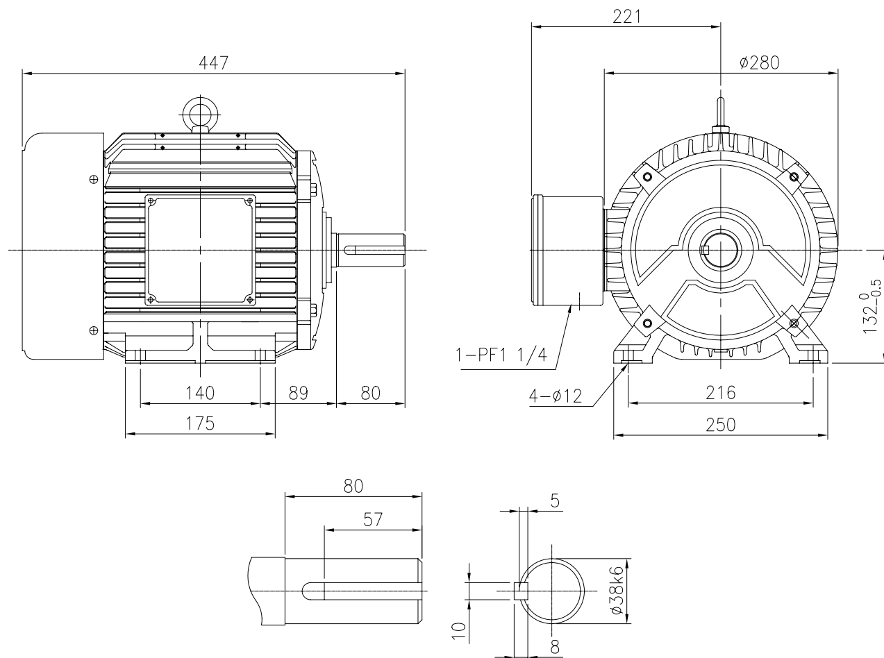
SHAFT EXTENSION
