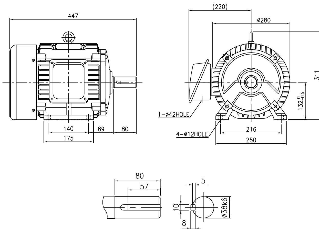
SHAFT EXTENSION
