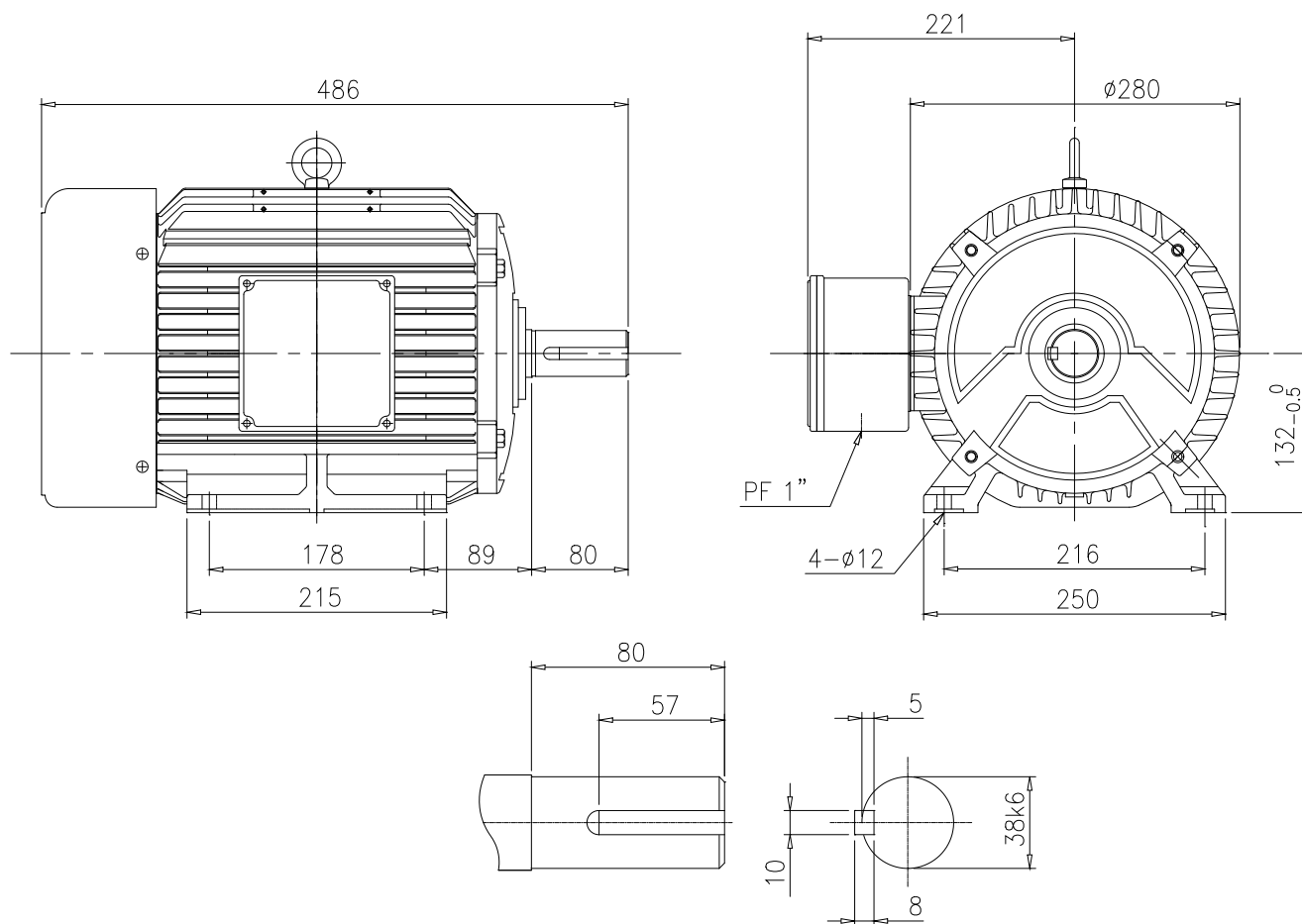
SHAFT EXTENSION
