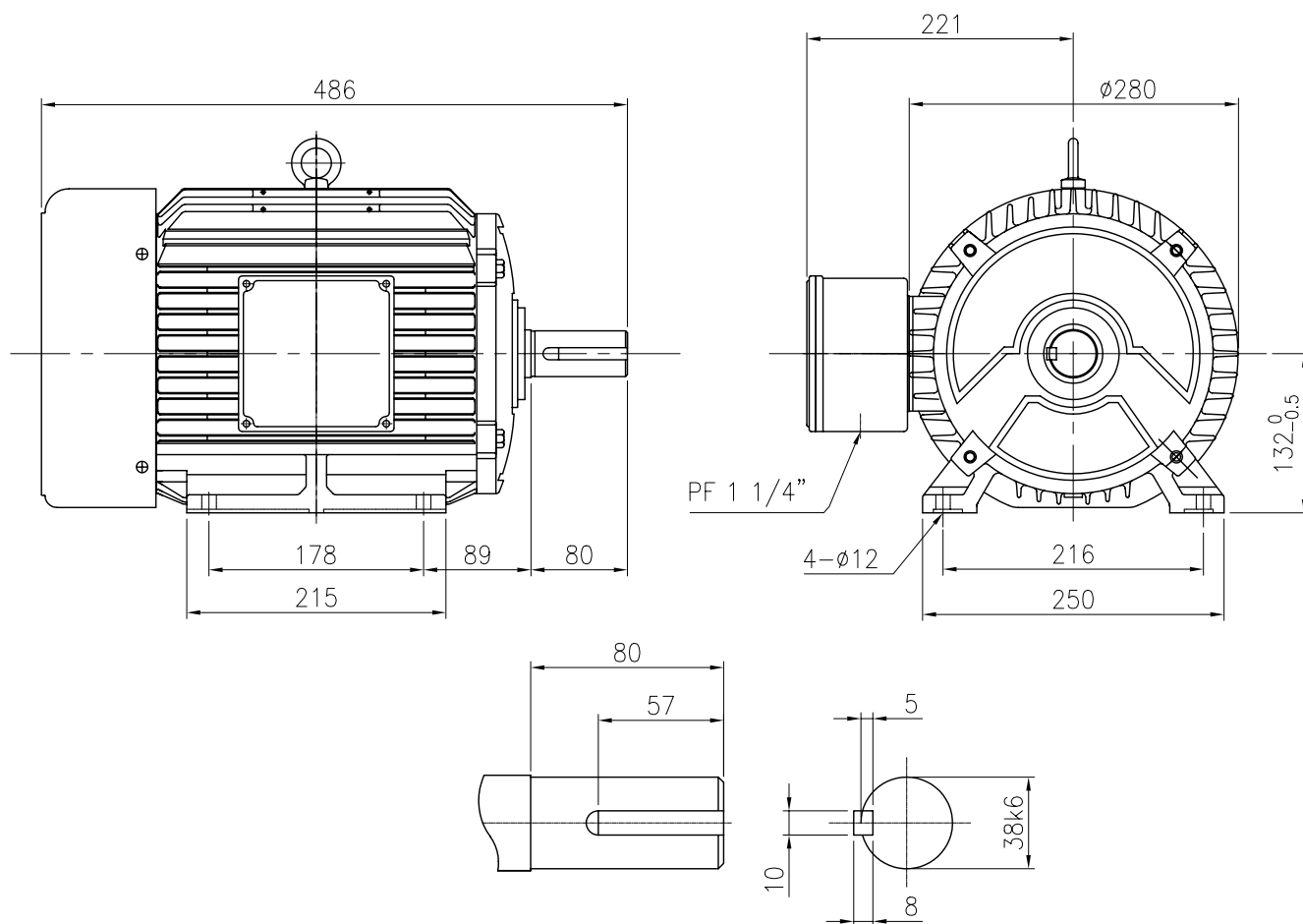
SHAFT EXTENSION
