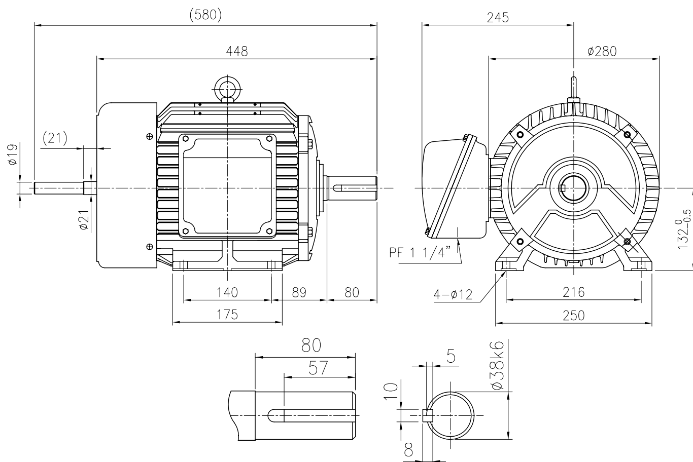
SHAFT EXTENSION
