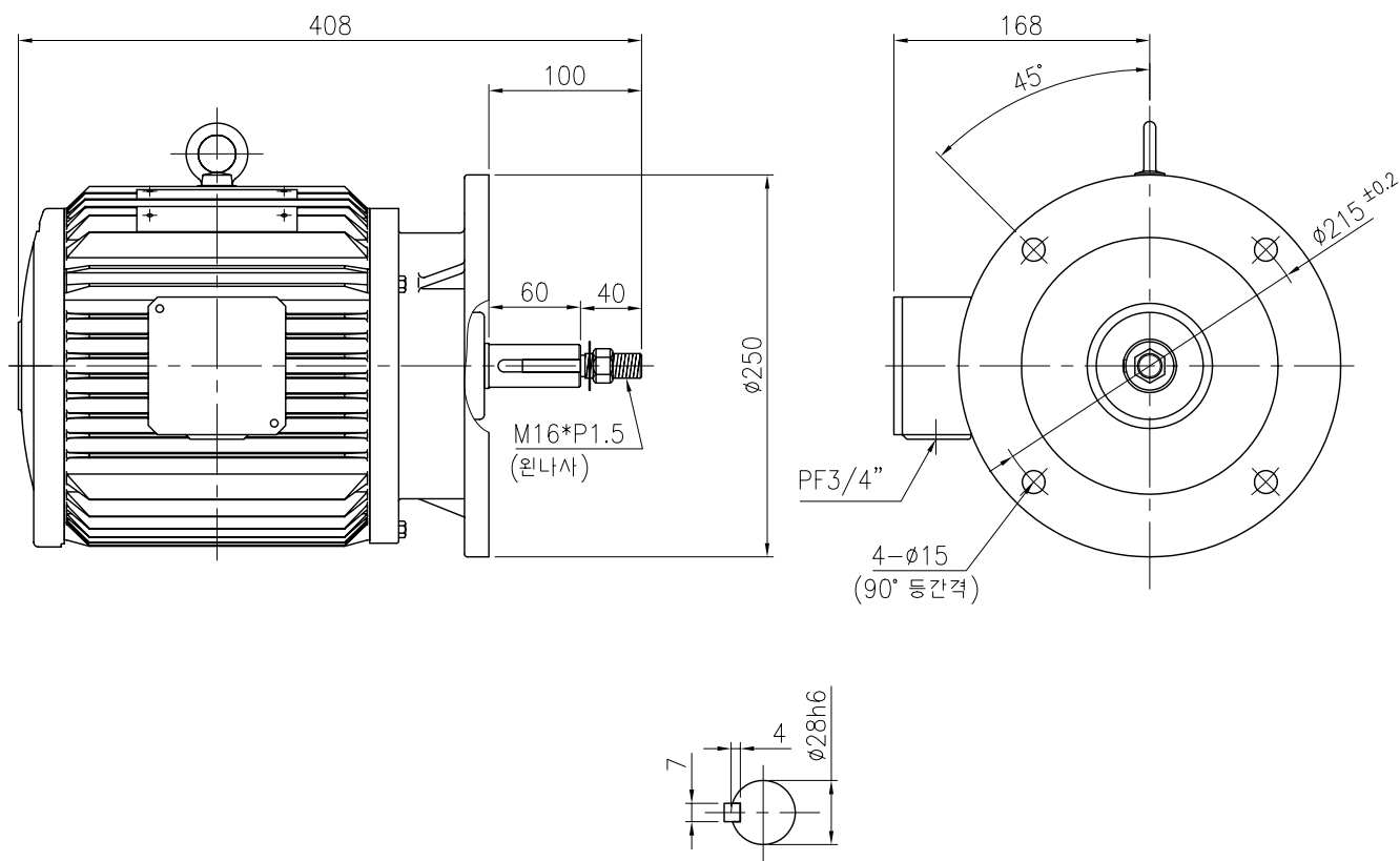
SHAFT EXTENSION
