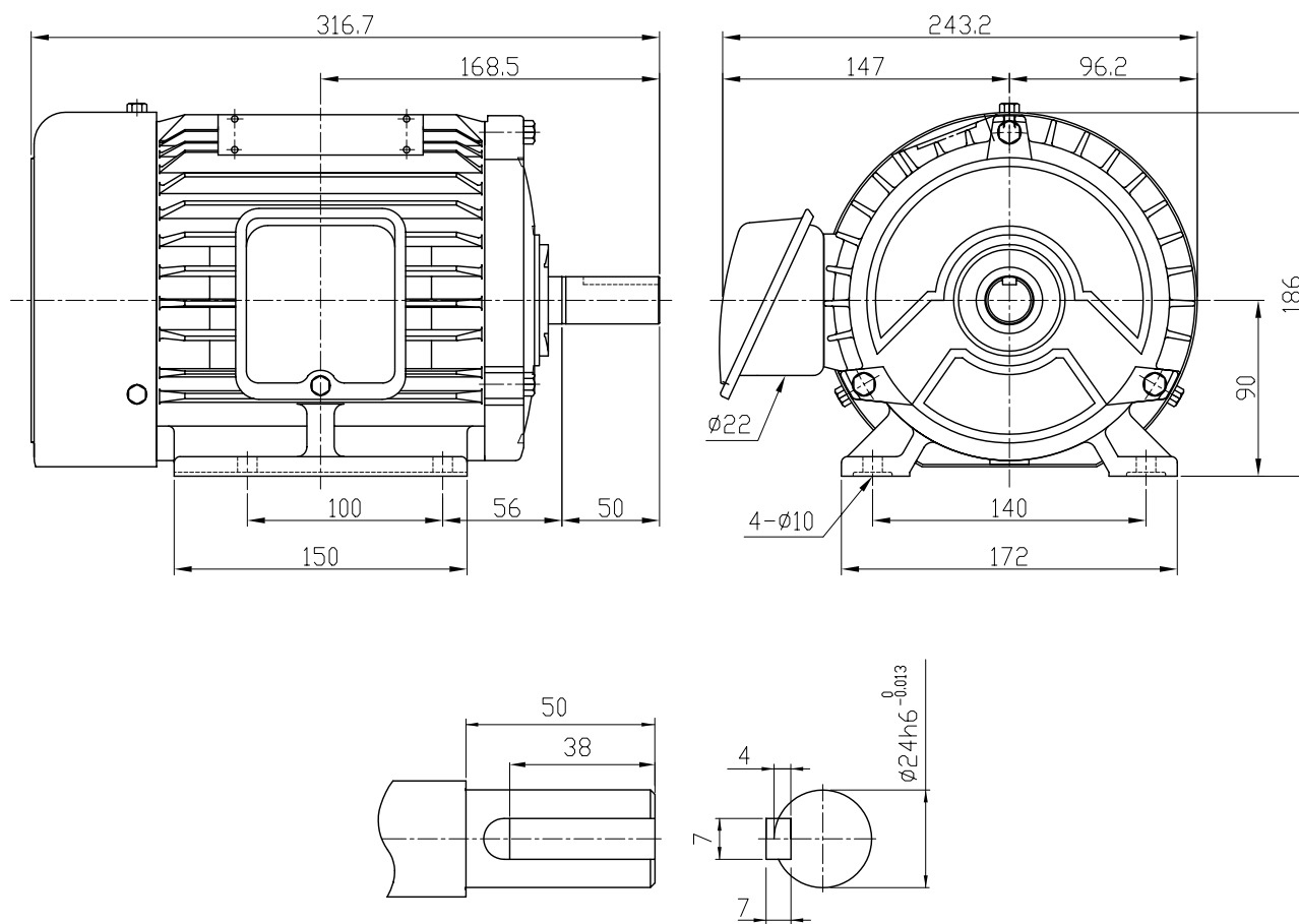
DETAIL OF SHAFT END
