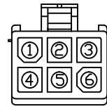
AMP 172168-1 PLUG 170360-1 PIN
