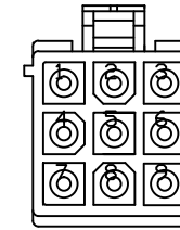
AMP 172169-1 PLUG 170359-1 PIN
