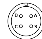
MS3102A20-4P Motor Cable Connector 접속도
